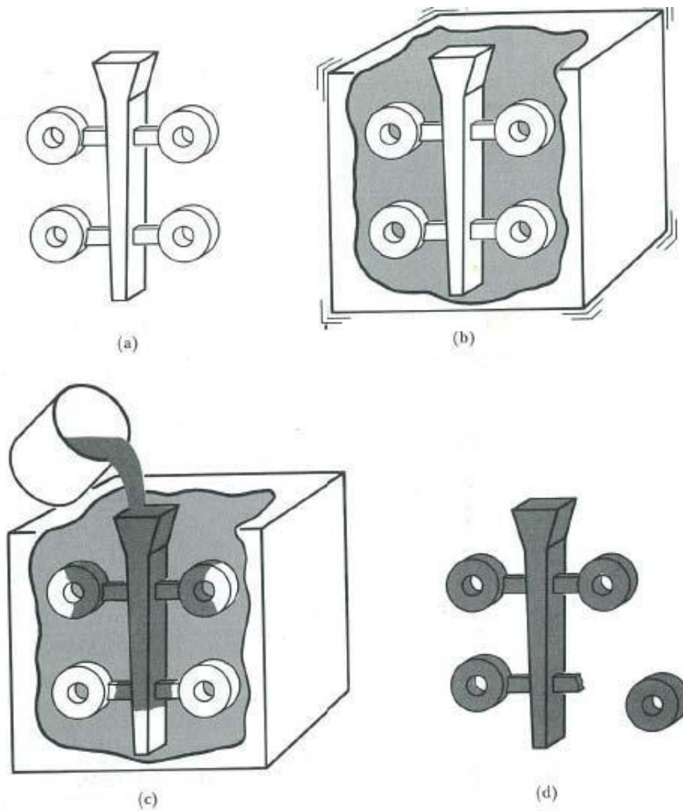
FIGURE 1-11 The evaporative pattern casting process involves the use of polymers and ceramics to produce a metal part. (a) An expanded polystyrene pattern is coated with ceramic, (b) the coated pattern is surrounded by vibrated sand, (c) molten metal vaporizes and displaces the Styrofoam, and (d) the solidified castings are removed from the tree and cleaned.
